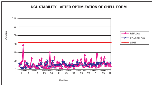
Figure 3: Optimization of shell form Reflow – Pressure cooker and lead-free reflow test DCL stability of B case
