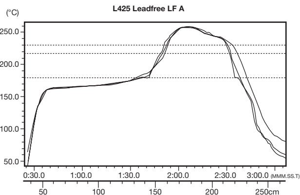
Figure 1: Lead-free profile
