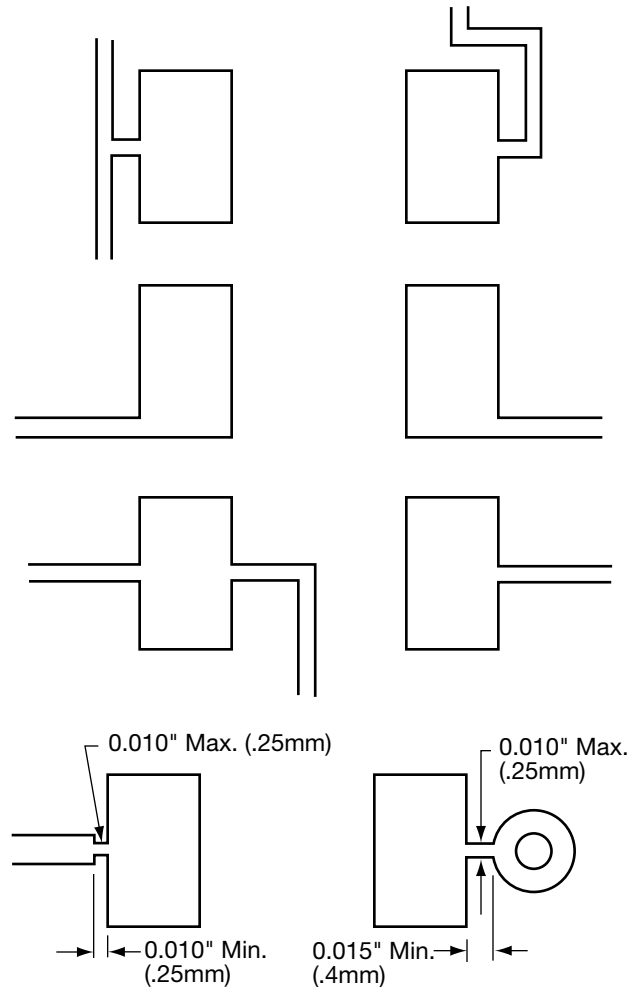
Figure 4. Design Techniques That Work
