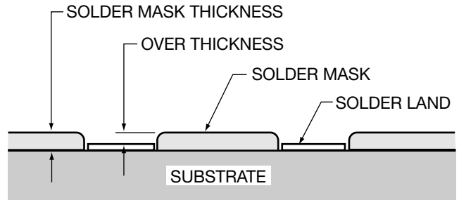
Figure 6. Solder Mask Overthickness
