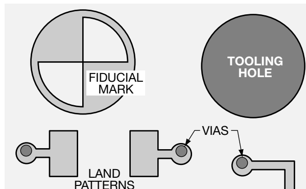
Figure 10. Tooling Holes Referenced to Artwork
