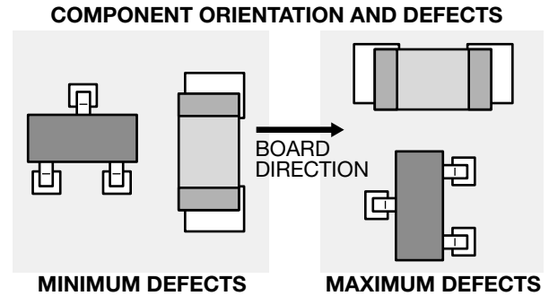
Figure 9. Component Orientation
