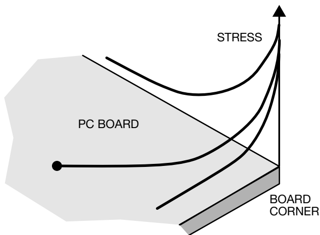
Figure 15. Stress Near a Board Corner
