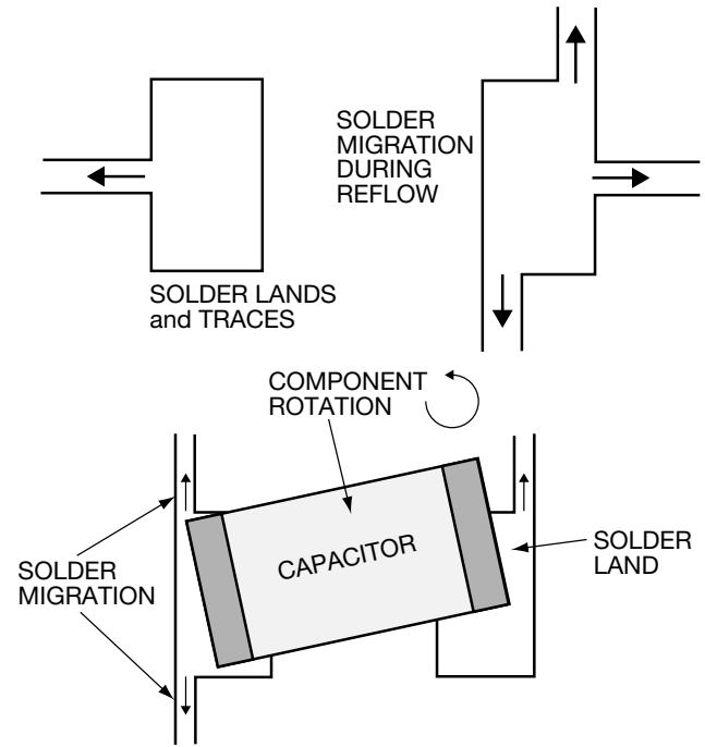
Figure 3. Design Techniques to Avoid
