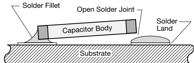
Figure 2. A Drawbridge
