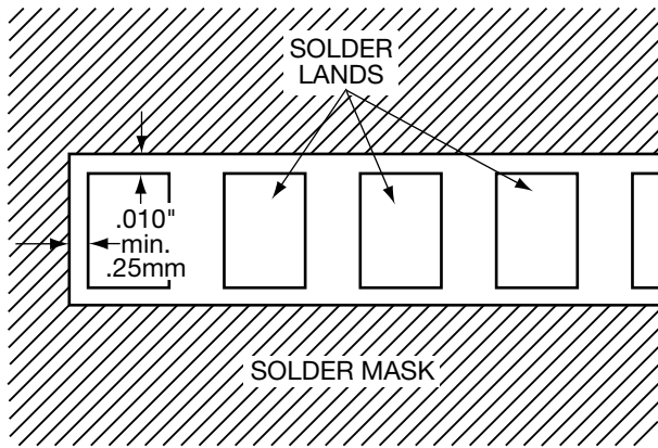
Figure 8. Recommended Solder Mask Windows
