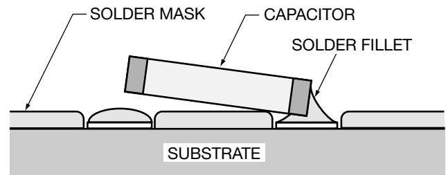
Figure 7. Resulting Induced Drawbridge
