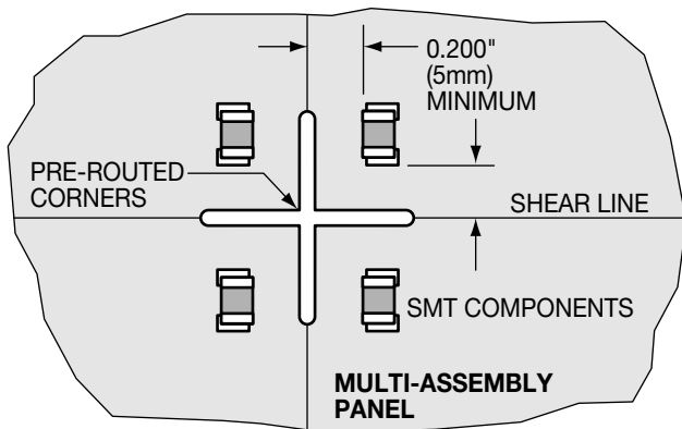
Figure 20. Pre-Routed Corners to Minimize Defects
