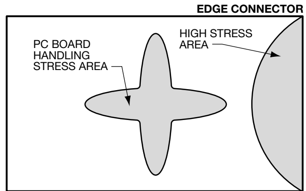
Figure 17. Board Bending and Connector Defect Zones
