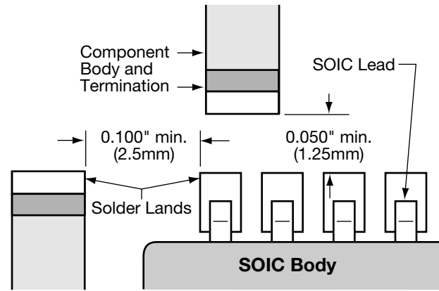
Figure 13. Chip to SOIC Spacing
