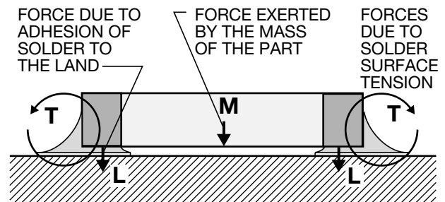
Figure 1. Defect and Counterdefect Forces
