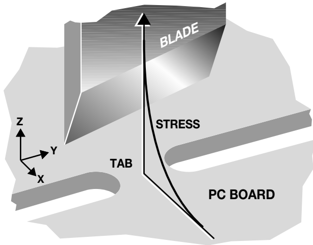
Figure 19. Tab Shearing Stress
