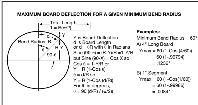
Figure 14. Bend Radius and Board Deflection
