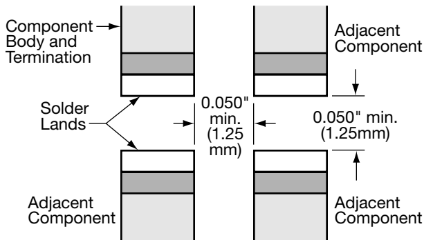
Figure 11. Chip Component Spacing
