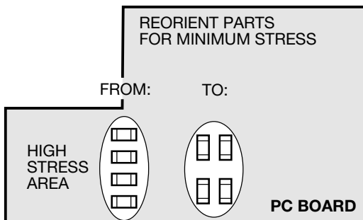
Figure 16. Orient Components for Minimum Stress
