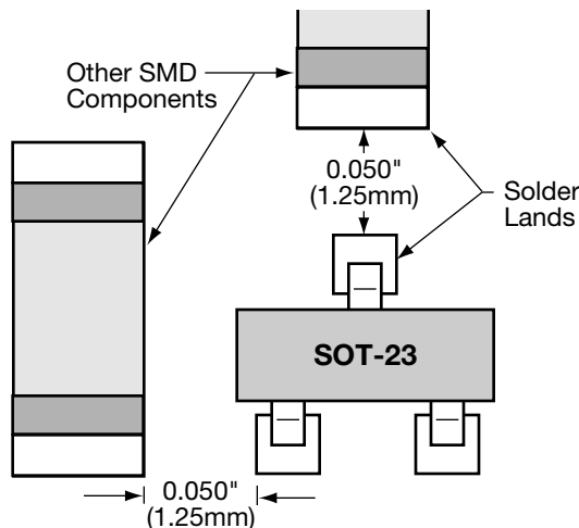
Figure 12. Chip to Transistor Spacing
