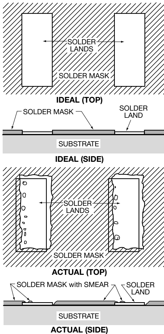
Figure 5. Ideal Solder Mask and the Result
