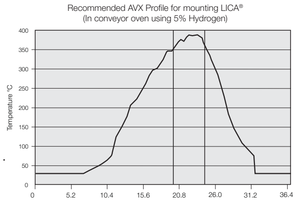
Figure 8. Typical Reflow Profile for LICA ® Capacitor
