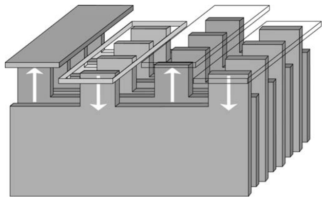
Figure 6. LICA's Electrode/Termination Construction The current path is minimized – this reduces self-inductance. Current flowing out of the positive plate, returns in the opposite direction along the adjacent negative plate - this reduces the mutual inductance.
