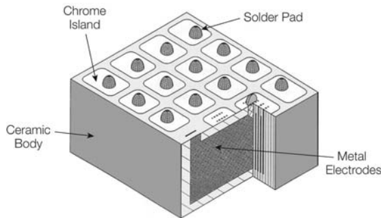
Figure 7. Cross Section of LICA ® Chip
