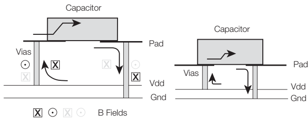
Figure 4. Inductance Developed in Current Loops
