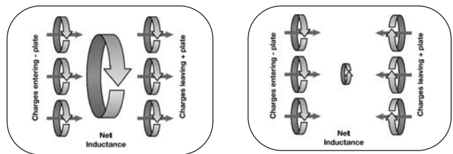
Figure 5. Net Inductance from Design
