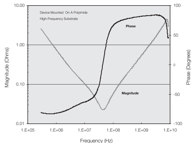
Figure 3. Typical Impedance and Phase curves for LICA ® 200nF Capacitor
